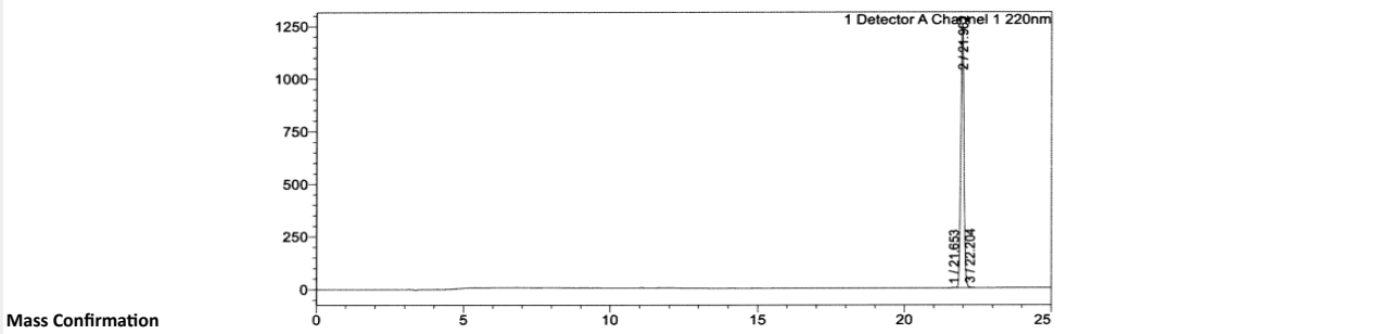
Mass Confirmation
